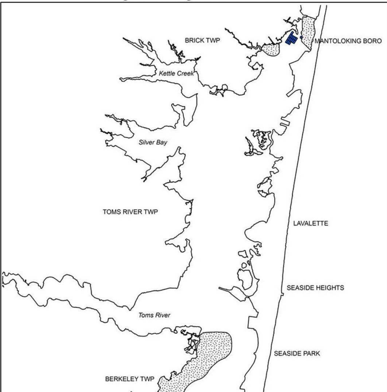
Hard clam distribution for upper Barnegat Bay, 2012. Areas without shading or coloring are read as "None."
