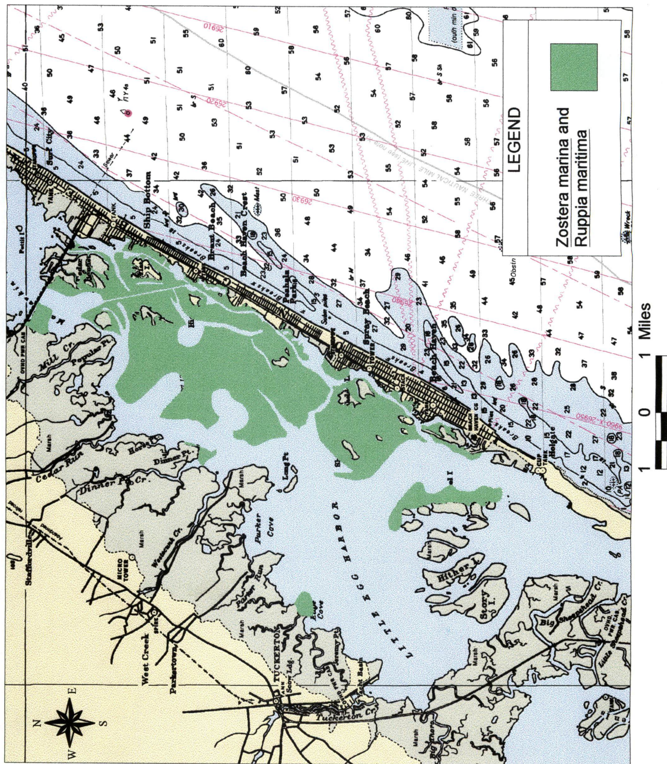
Figure 5. 2001 Little Egg Harbor Bay Shellfish Inventory: SAV distribution.
