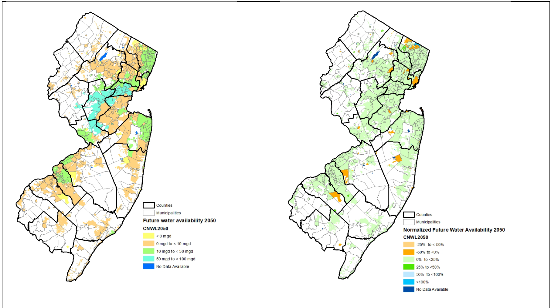
Figure K4a. (left) shows the projected 2050 water availability by public water system for the Conservation Nominal Water Loss Scenario (CNWL). Figure K4b. (right) shows the projected 2050 water availability normalized by 2021 average daily demand for the CNWL scenario.
