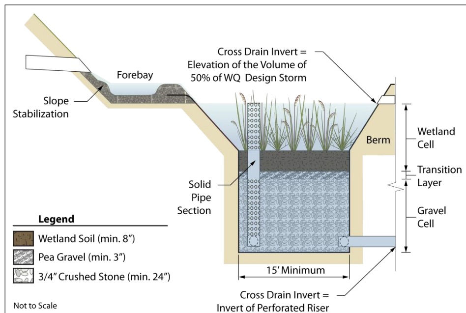
Detailed Profile of Wetland Cell #1 and Gravel Cell #1
