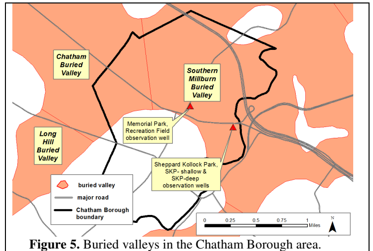
Figure 5. Buried valleys in the Chatham Borough area.
