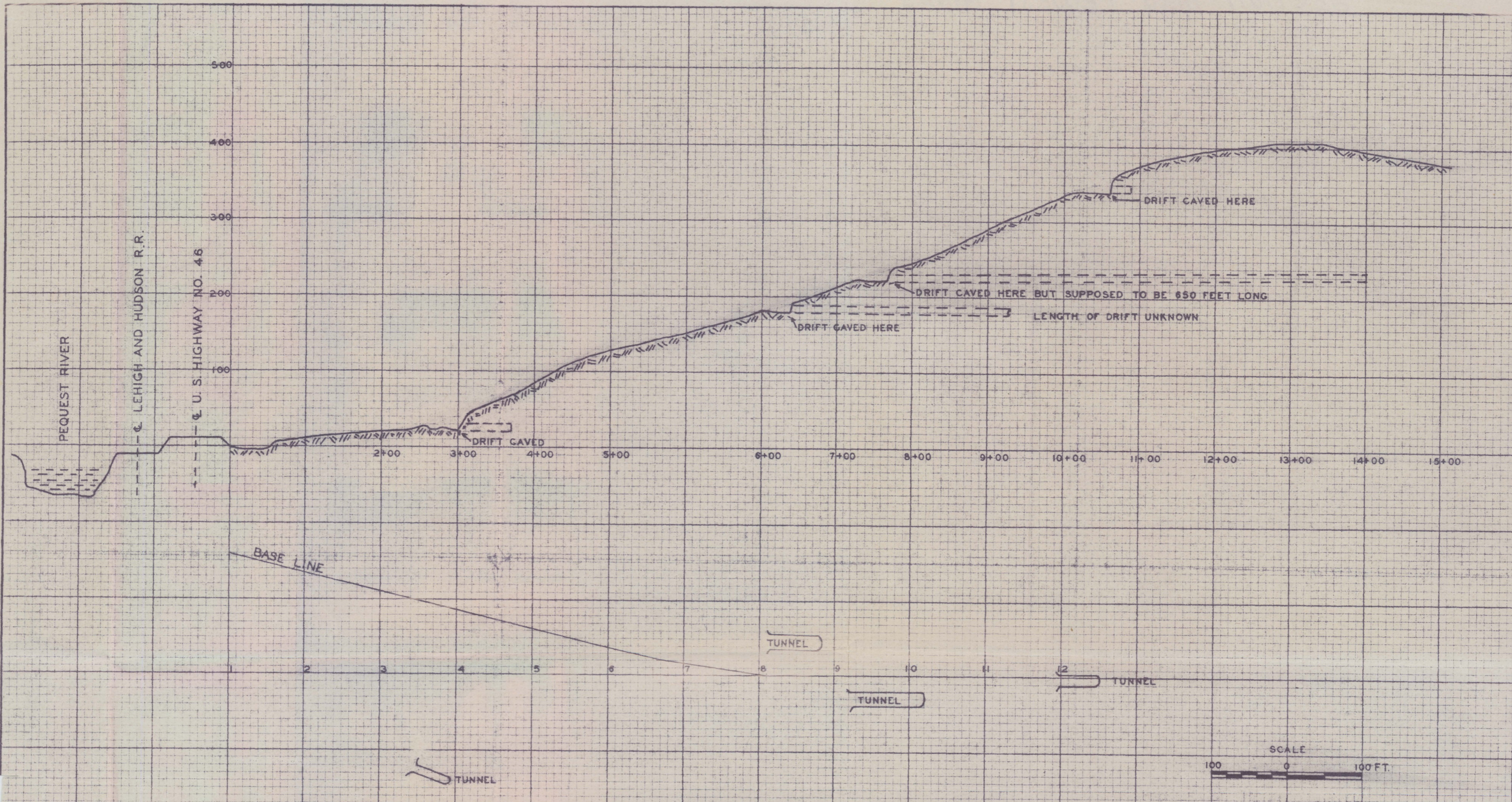
FIG. 4 SECTION "A" - "A" LOOKING SOUTH HENRY TUNNEL
