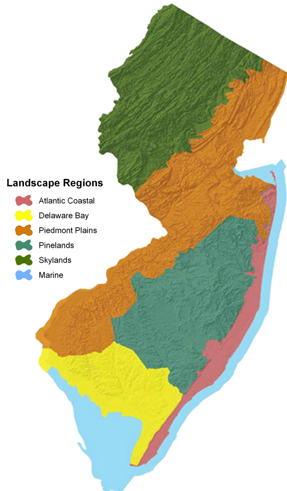
New Jersey's Landscape Regions
