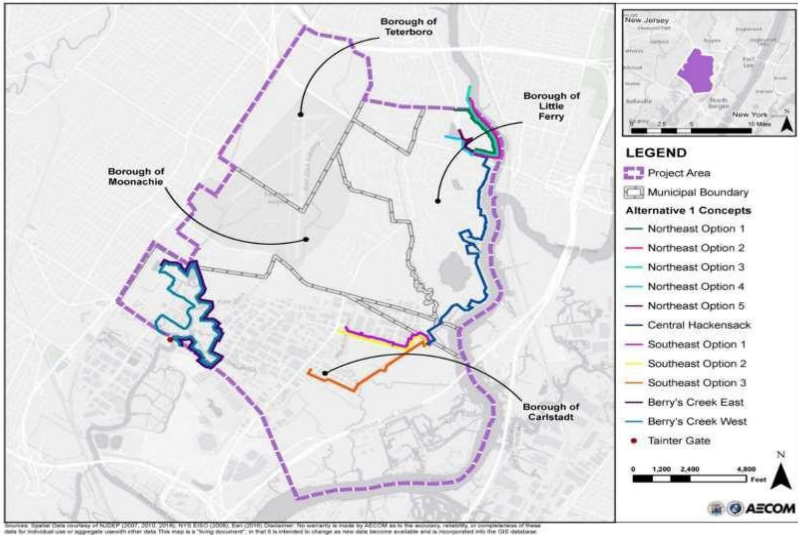
Potential Alignments within Alternative 1 Line of Protection
