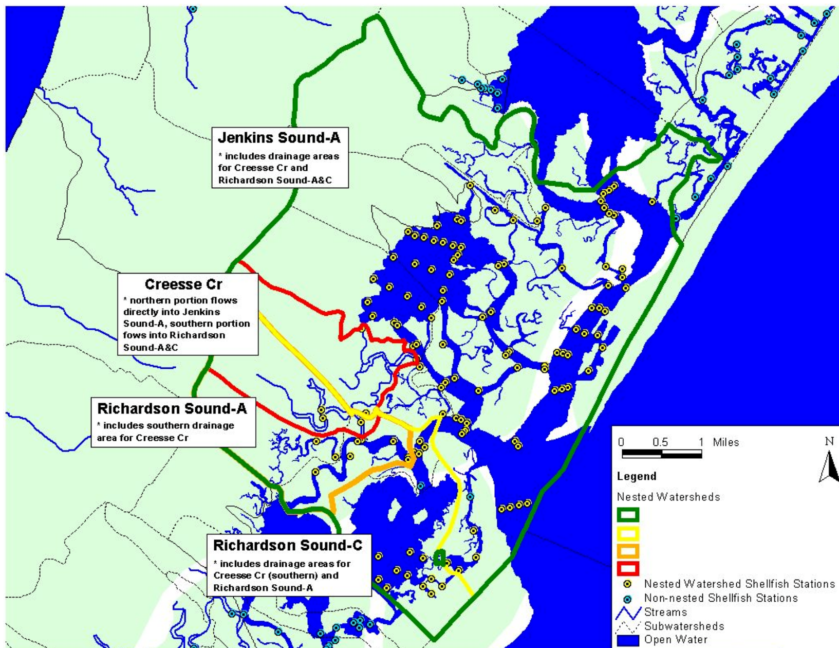
E1. Cresse Creek Estuary, Jenkins Sound-A, Richardson Sound-A, and Richardson Sound-C (WMA 16)
