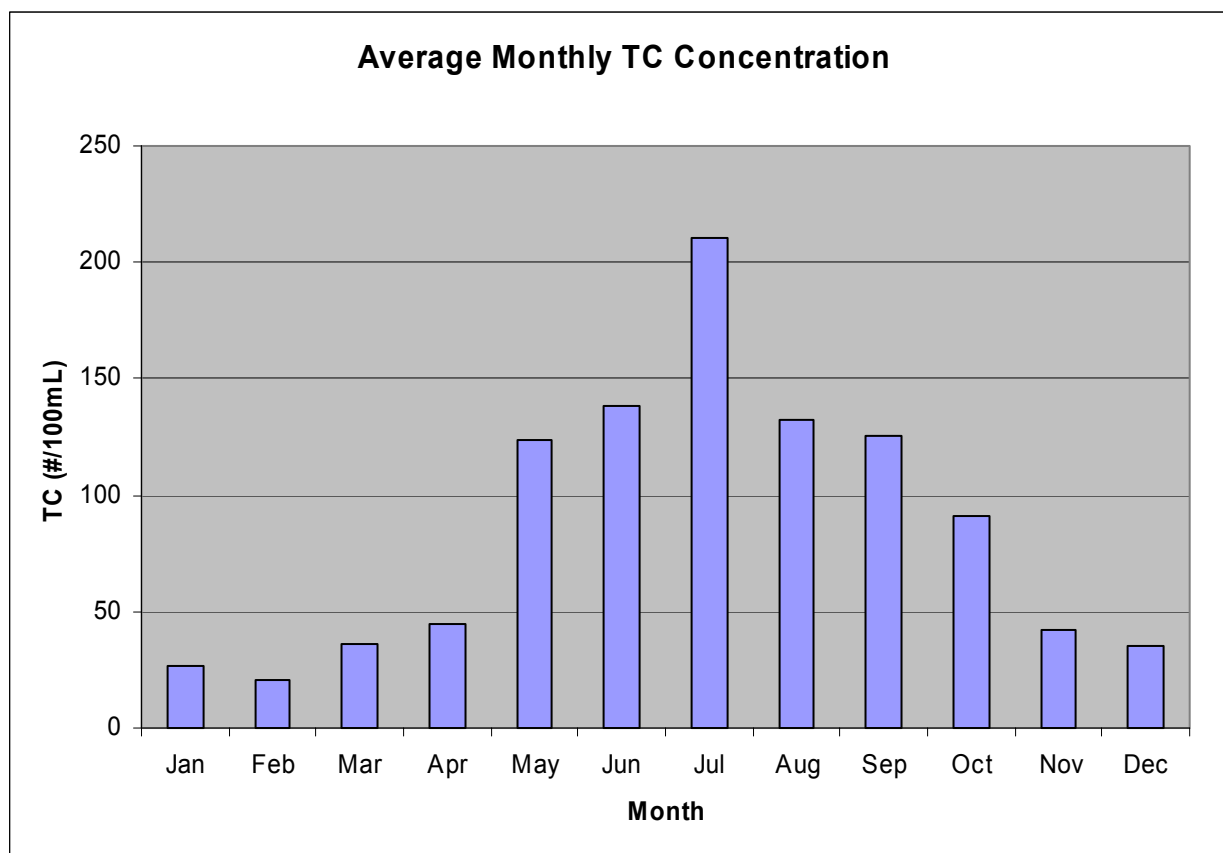
Figure 4. Seasonal trend in TC data for all worst case stations in WMA 16
