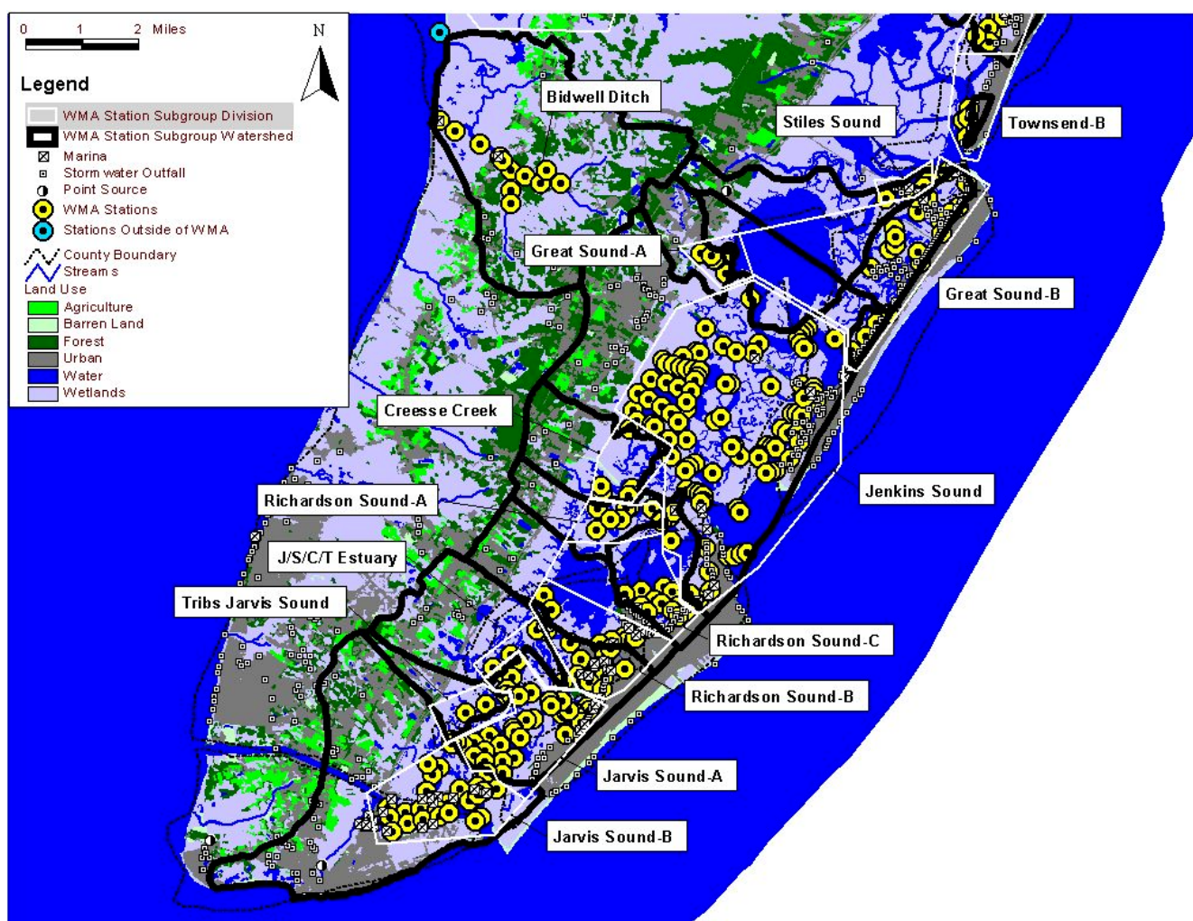
Figure 3. Primary pathogen indicator source data used in TMDL development for southeastern portions of WMA 16
