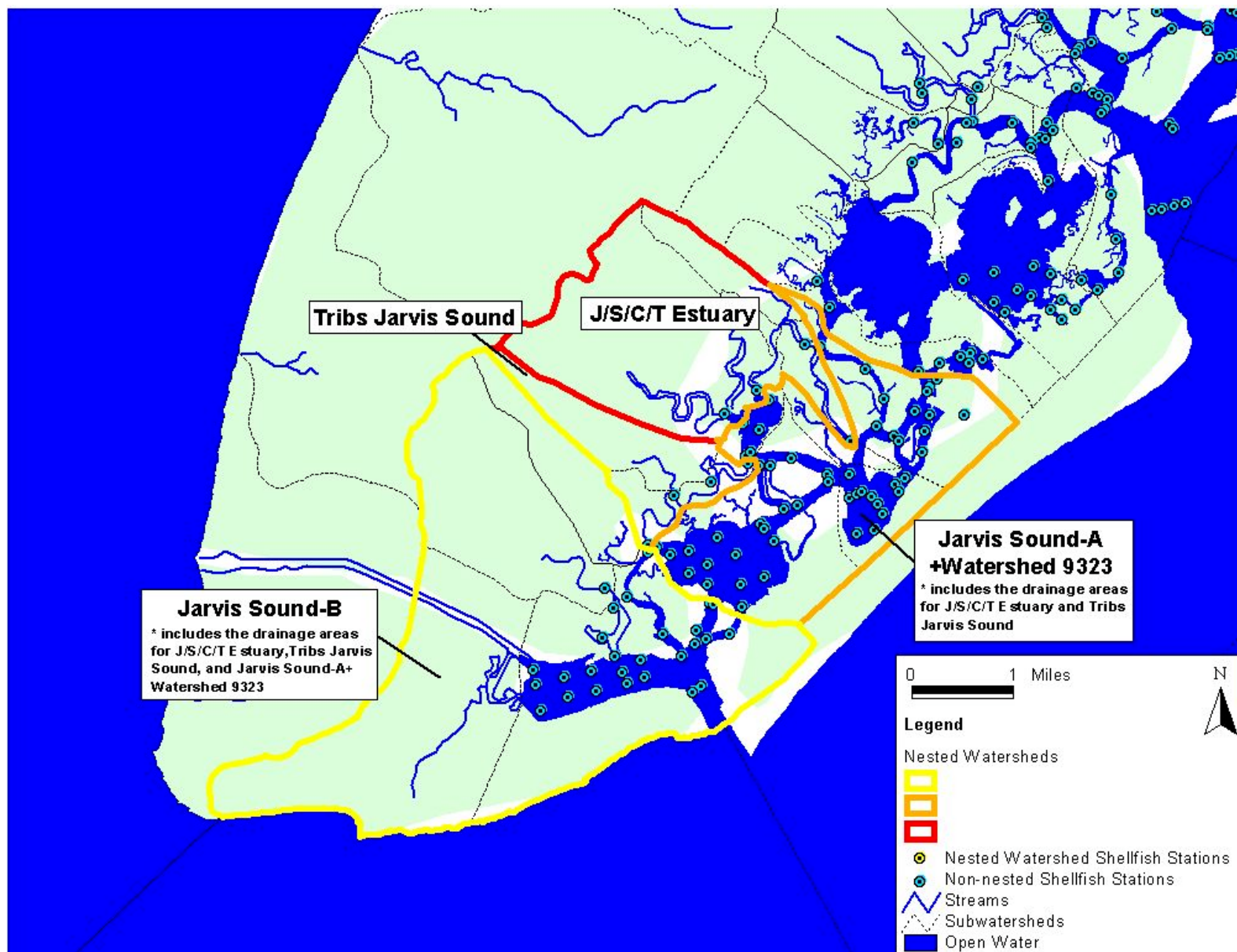
E2. Jones/Stites/Carino/Taylor Estuary, Tribes Jarvis Sound, Jarvis Sound-A+Richardson Sound-B (Watershed #9323), and Jarvis Sound-B Nested Watersheds (WMA 16)
