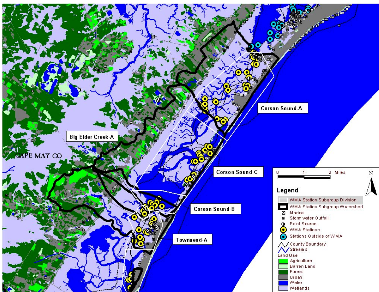
Figure 2. Primary pathogen indicator source data used in TMDL development for northeastern portions of WMA 16
