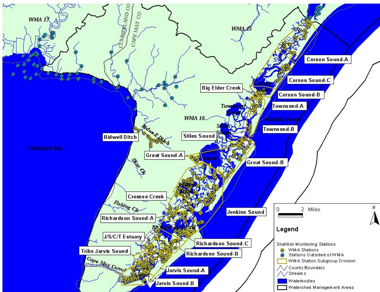
Figure 1. Shellfish impaired waterbodies in WMA 16
