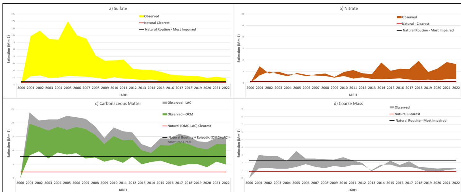
Figure D-7. Range of Observed and Estimated Natural Light Extinction for Select Individual Species at James River Face on 20 Percent Clearest and Most Impaired Visibility Days
