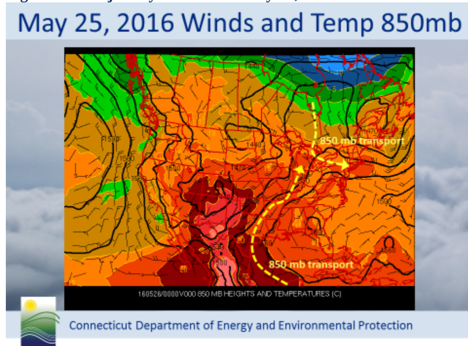
Figure 30: Trajectory of Wind on May 25, 2016
