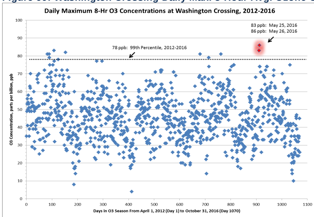
Figure 99: Washington Crossing Daily Max. 8-Hour Avg. Ozone Conc.
