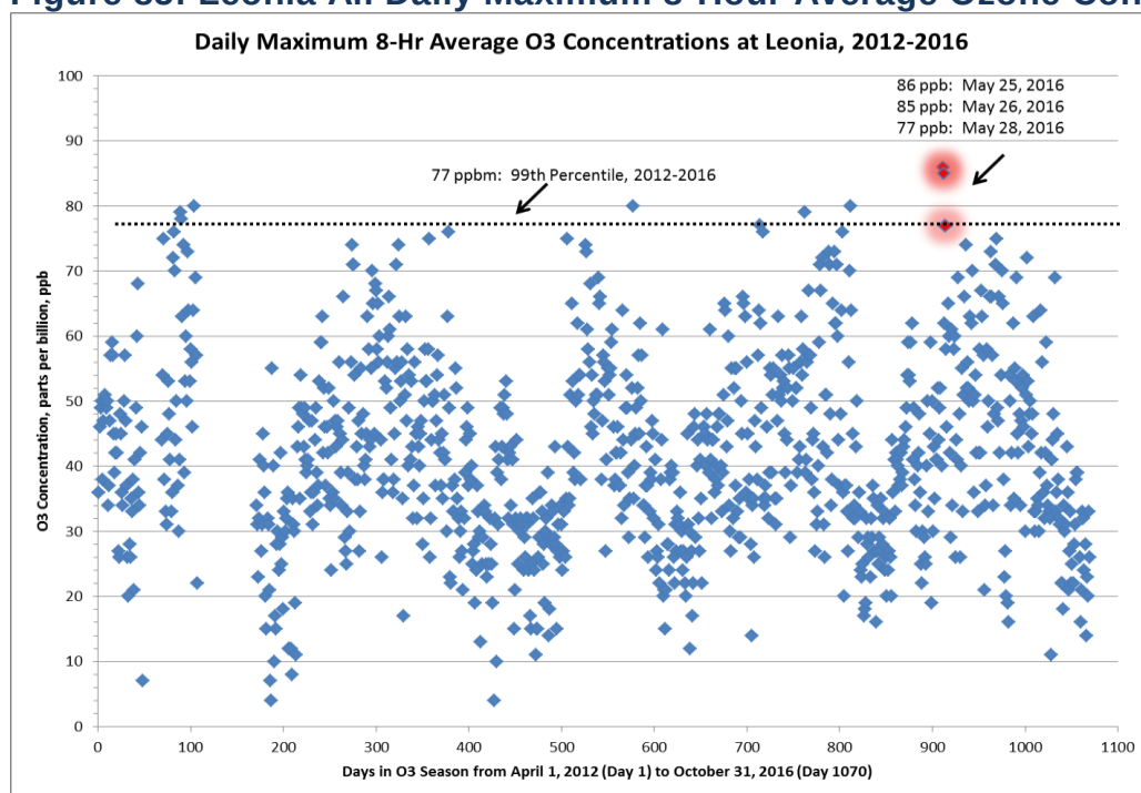
Figure 85: Leonia All Daily Maximum 8-Hour Average Ozone Concentrations
