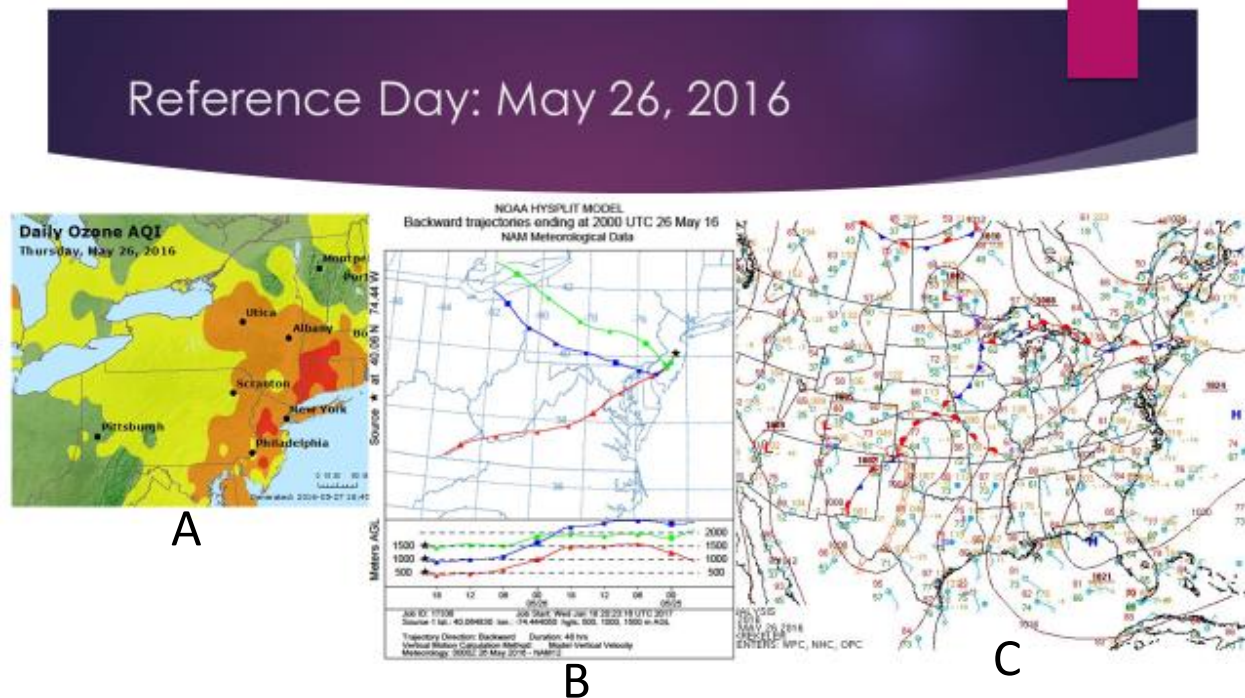
Figure 44: May 26, 2016 Reference Day Weather Patterns
