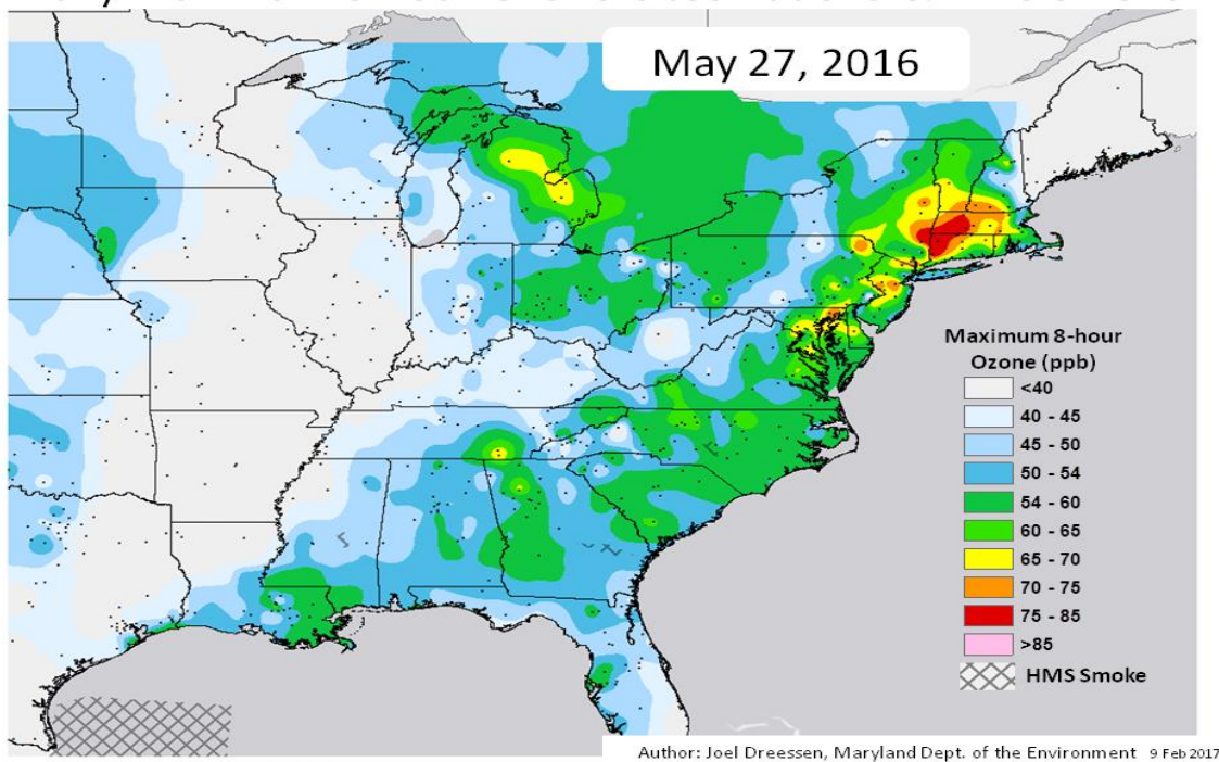
Figure 117: Overlay of Smoke Plume and Ozone Levels, May 27, 2016 Daily Maximum 8-hour Ozone Observations & HMS Smoke
