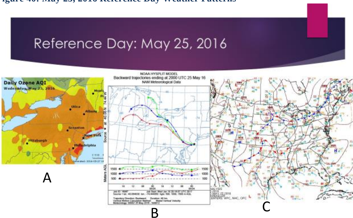
Figure 40: May 25, 2016 Reference Day Weather Patterns
