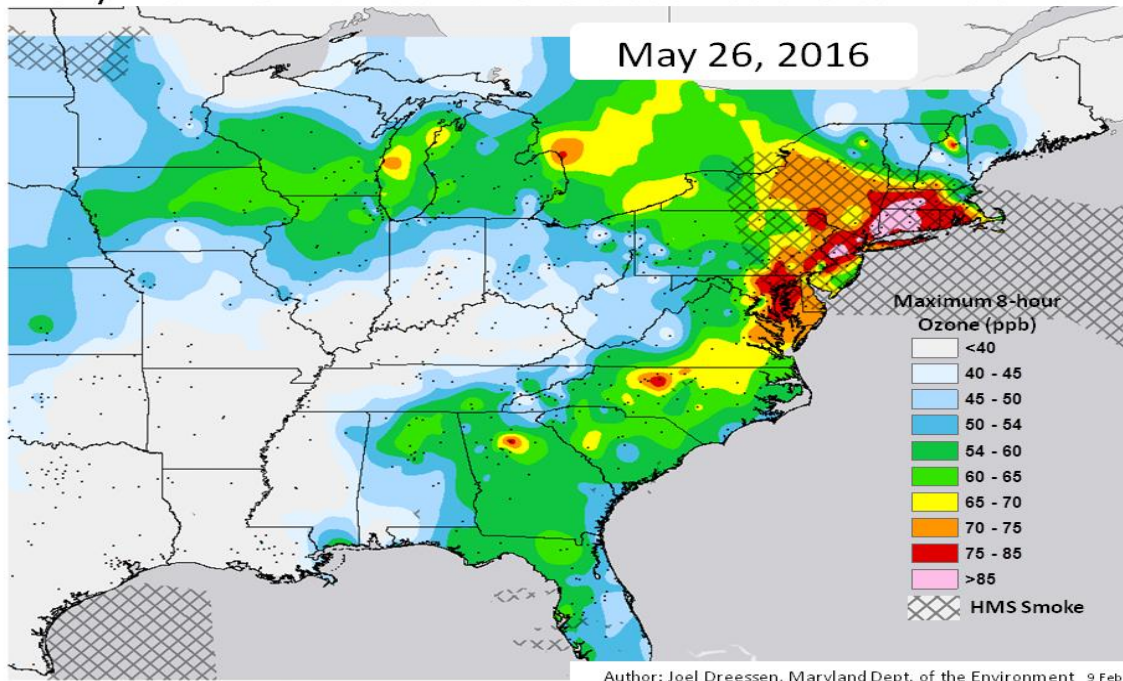
Figure 116: Overlay of Smoke Plume and Ozone Levels, May 26, 2016 Daily Maximum 8-hour Ozone Observations & HMS Smoke
