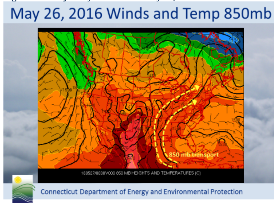
Figure 33: Trajectory of Wind on May 26, 2016
