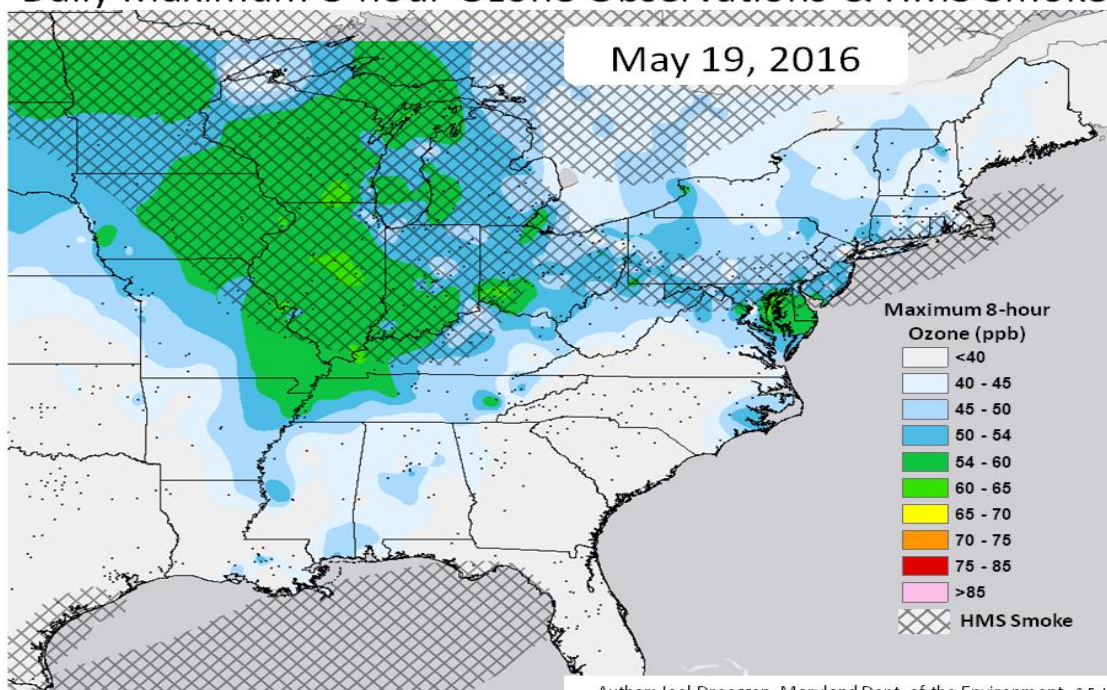
Figure 109: Overlay of Smoke Plume and Ozone Levels, May 19, 2016
