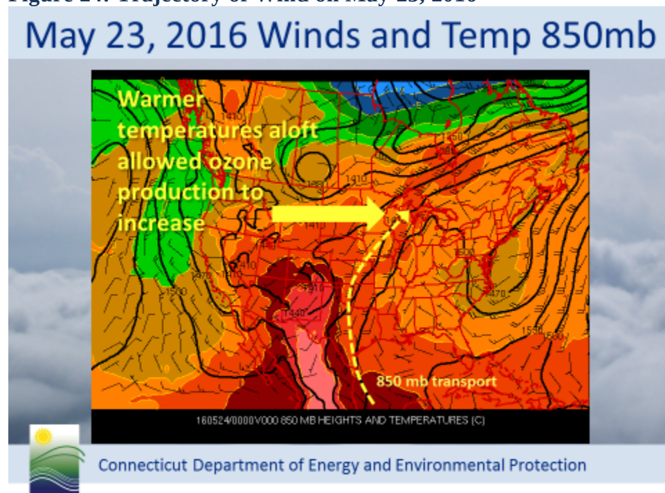
Figure 24: Trajectory of Wind on May 23, 2016
