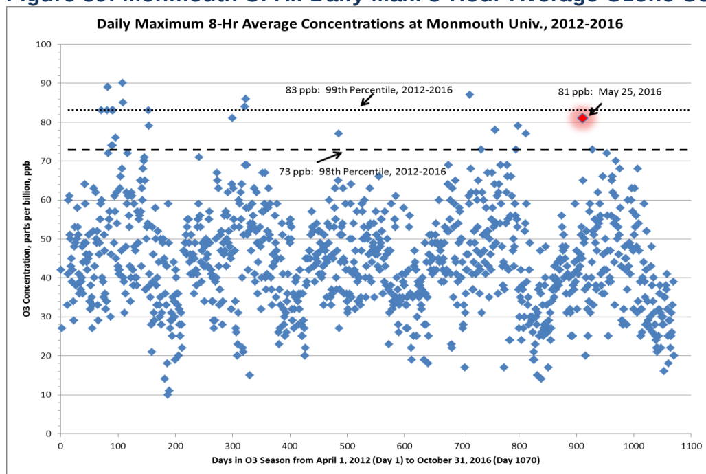
Figure 89: Monmouth U. All Daily Max. 8-Hour Average Ozone Concentrations
