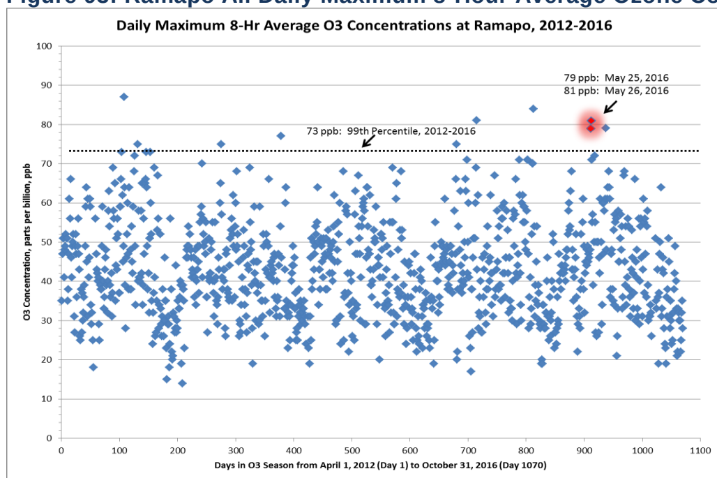
Figure 93: Ramapo All Daily Maximum 8-Hour Average Ozone Concentrations
