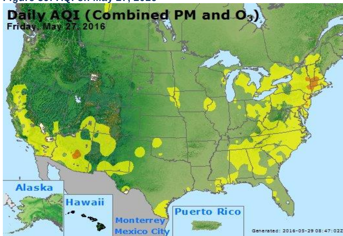
Figure 59: AQI on May 27, 2016
