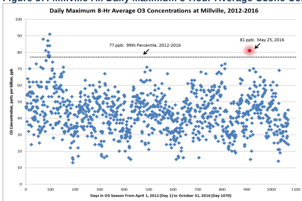
Figure 87: Millville All Daily Maximum 8-Hour Average Ozone Concentrations
