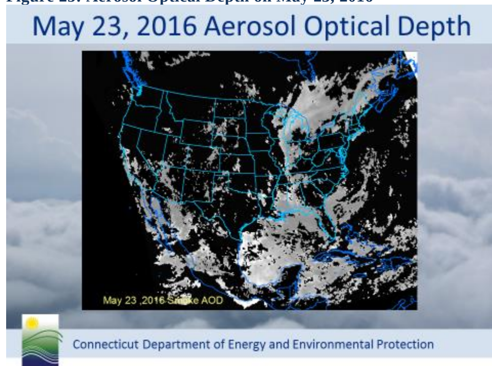
Figure 25: Aerosol Optical Depth on May 23, 2016
