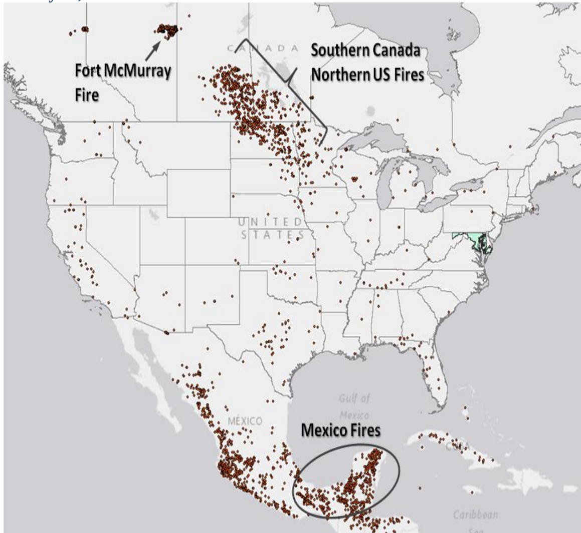
Figure 107: The Location of All Wildfires in the U.S., Mexico, and Canada from May 17 to May 20, 2016
