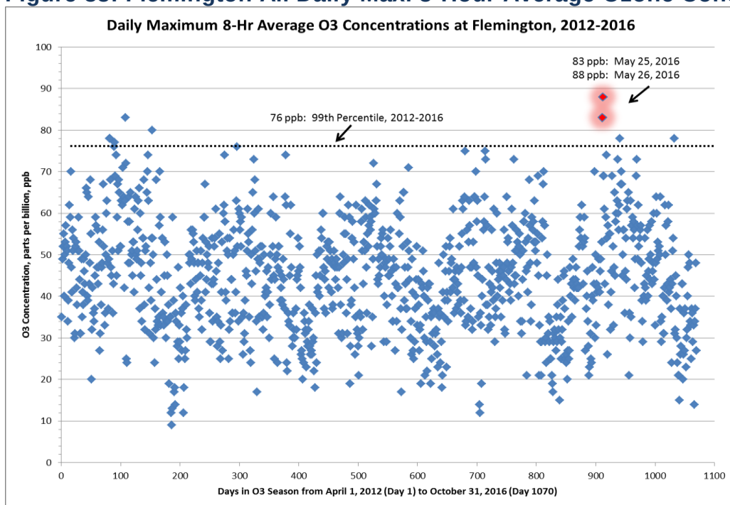
Figure 83: Flemington All Daily Max. 8-Hour Average Ozone Concentrations
