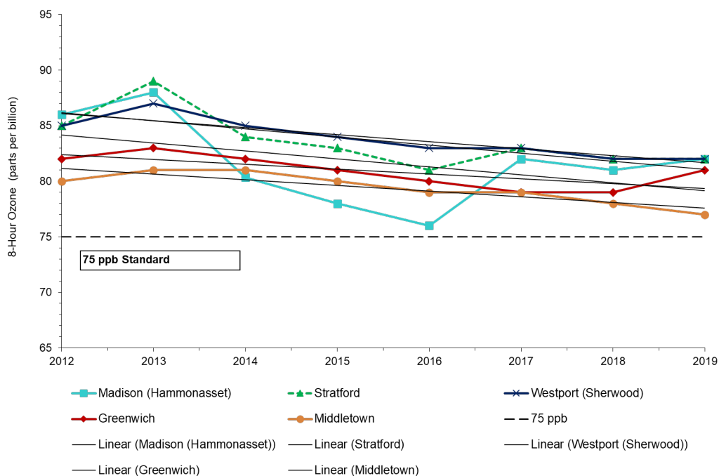
Figure A2-2.2: 8-hour Ozone Design Values 2012-2019 The 5 Monitors Exceeding 75 ppb Ozone NAAQS Northern NJ-NY-CT Nonattainment Area
