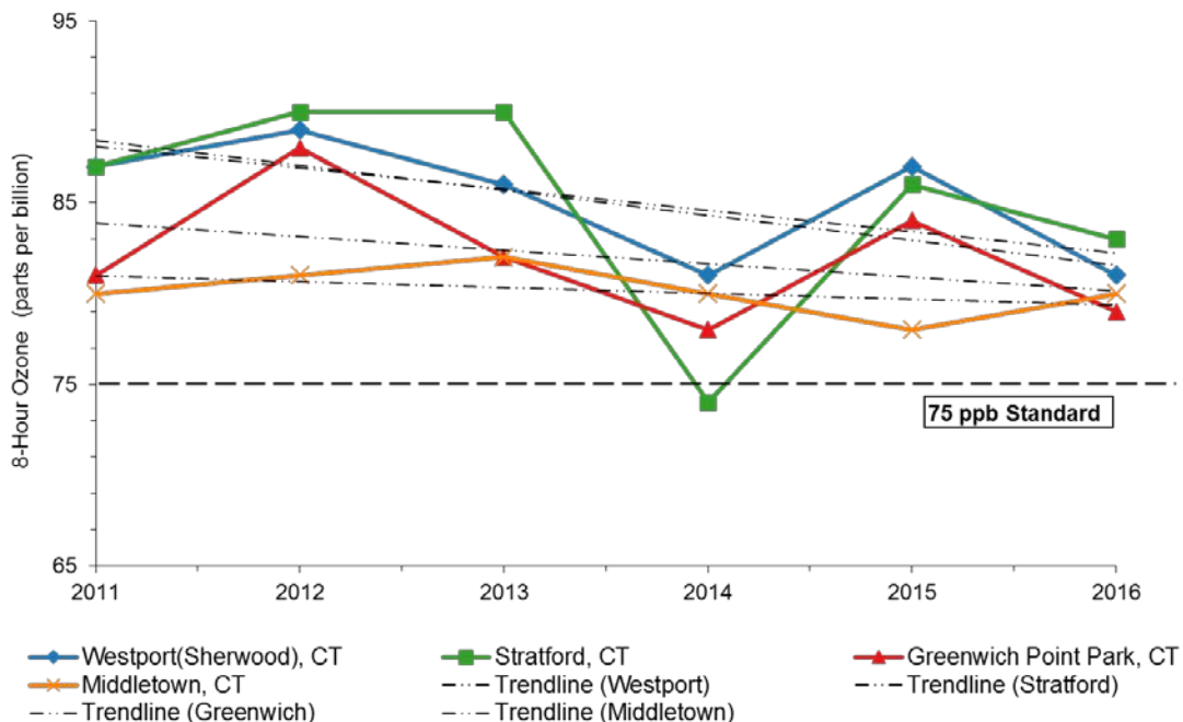
Figure A2-2.8: 8-hour Ozone 4th Highest Daily 8-Hour Maximum 2011-2016 Next 4 Monitors Exceeding 75 ppb Ozone NAAQS Northern NJ-NY-CT Nonattainment Area
