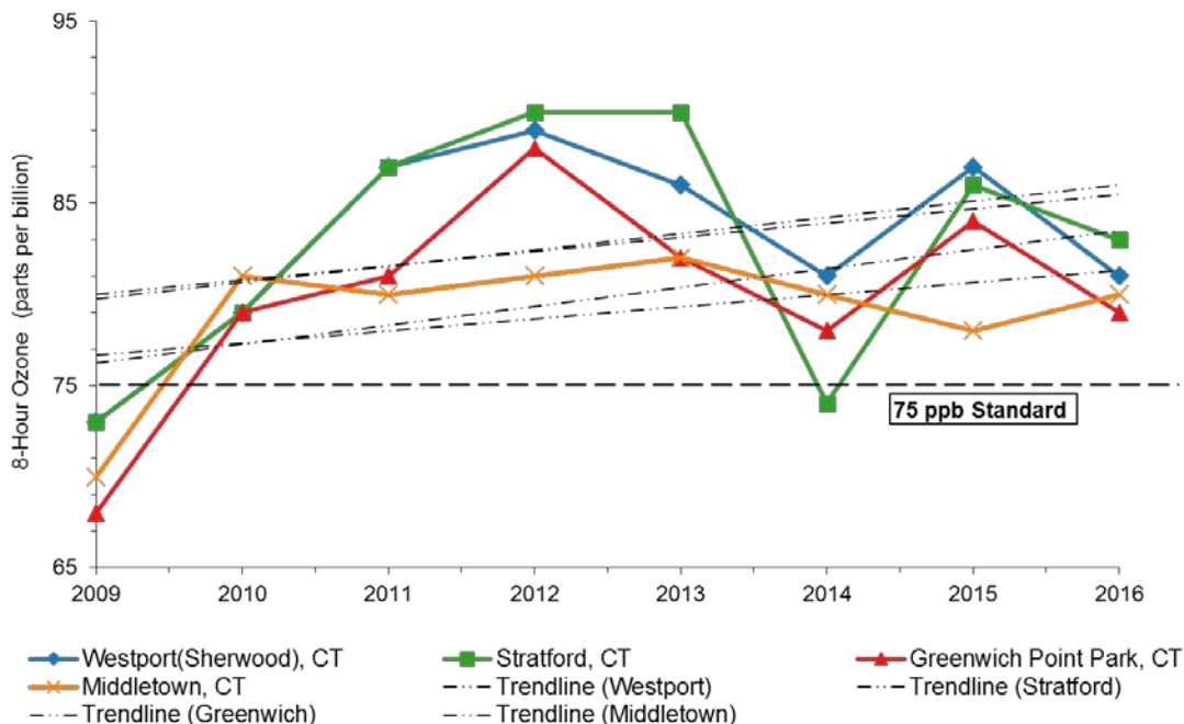
Figure A2-2.6: 8-hour Ozone 4th Highest Daily 8-Hour Maximum 2009-2016 Next 4 Monitors Exceeding 75 ppb Ozone NAAQS Northern NJ-NY-CT Nonattainment Area
