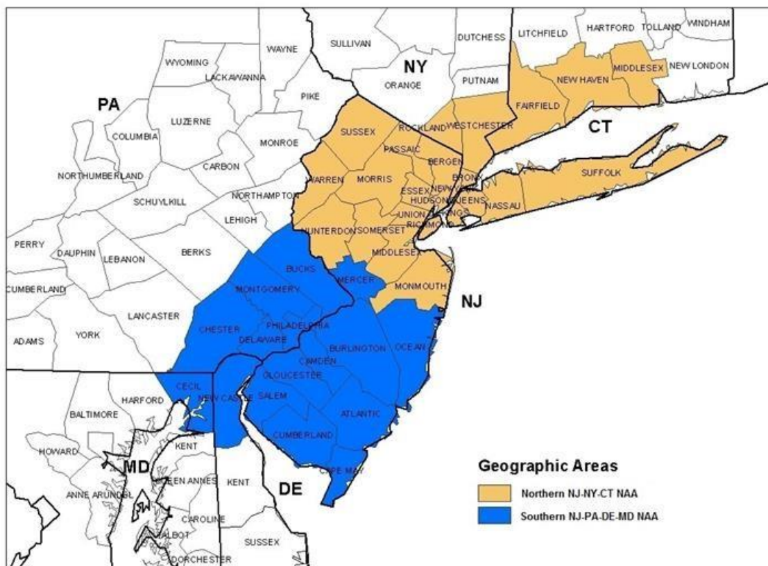
Figure 10-1: New Jersey 8-Hour Ozone Nonattainment Areas (NAA) 75 and 70 ppb NAAQS
