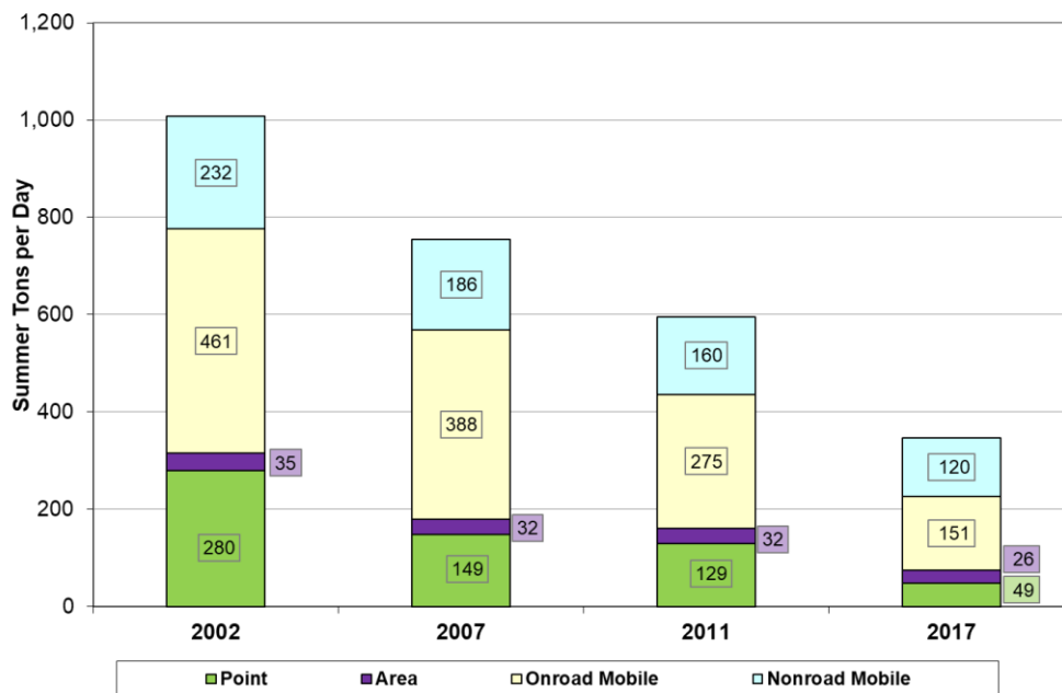
Figure 10-16: New Jersey Statewide Nitrogen Oxides Emission Trend
