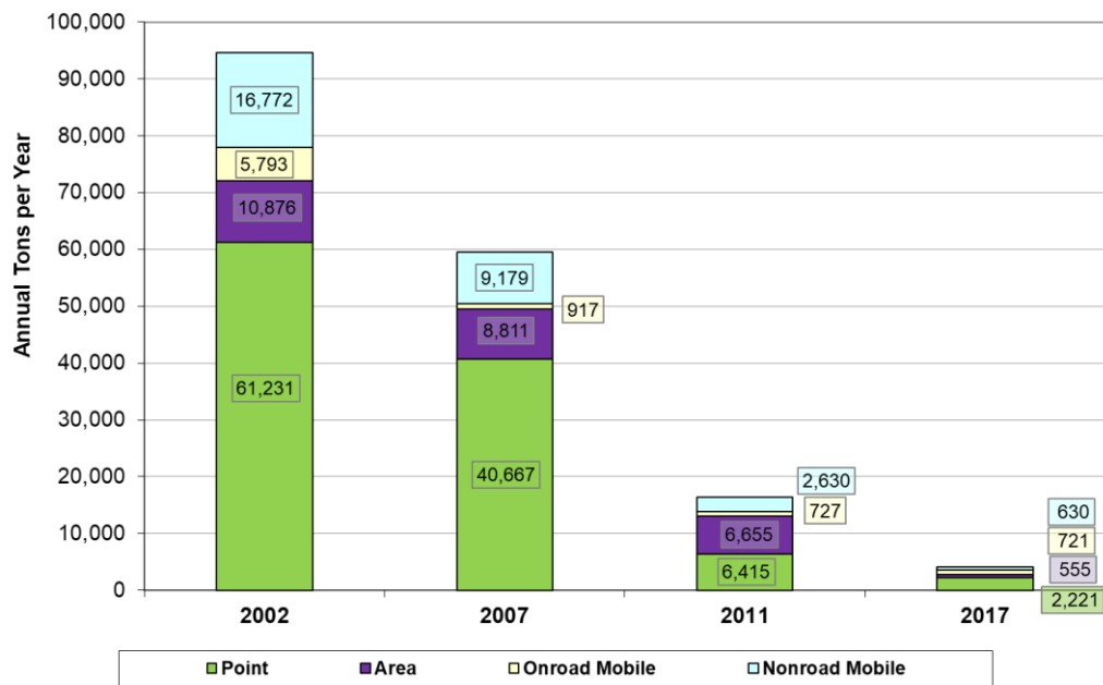
Figure 10-20: New Jersey Statewide Ammonia Emission Trend
