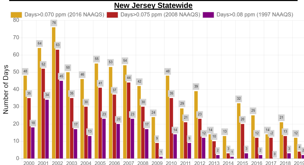
Figure 2-6: Number of Days the 8-Hour Ozone Standard was Exceeded 2000-2019
