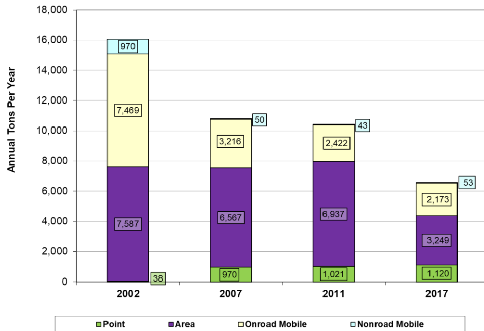
Figure 10-20: New Jersey Statewide Ammonia Emission Trend
