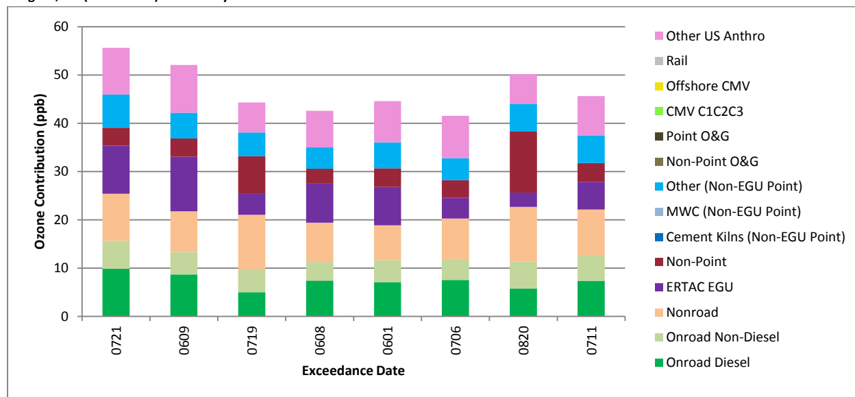
Figure 13-5: Anthropogenic US intra-domain contribution by sector on dates projected to exceed the 70 ppb NAAQS in 2023 to Susan Wagner, NY (360850067) ordered by total DVF
