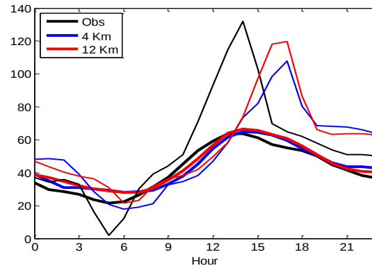
Figure 7-17: Observed and modeled (4km/12km grids) ozone (ppb) for July 2011 at monitor #090013007 (thick line: monthly avg., thin line: max day)
