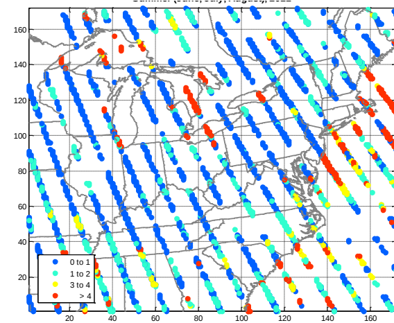
Figure 2-24: CALIPSO to WRF (PBL height ratio) Summer (J/J/A) 2011
