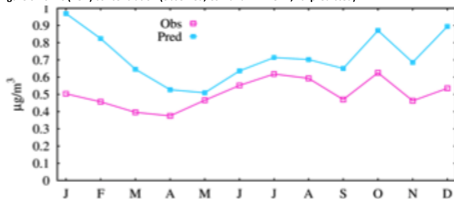
Figure 6-46: EC (TOR) concentration (observed, CSN and IMPROVE, vs. predicted)
